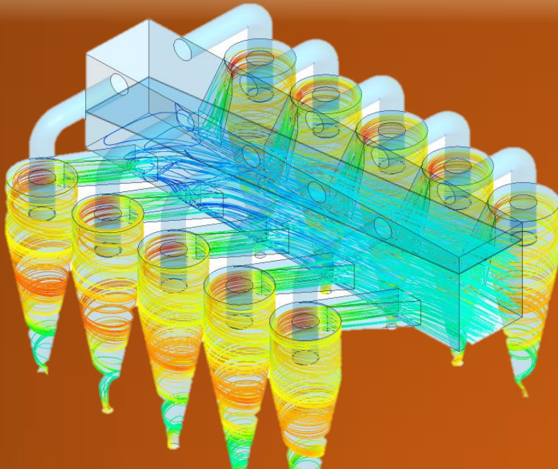
CFD investigation of a cyclone separator system conducted for CIMPEX Pvt. Ltd.
