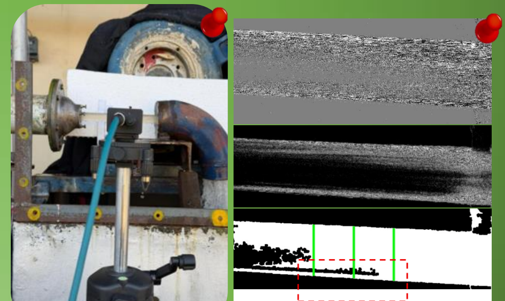
Works related to jet flow visualization using event based camera at TTL by undergraduate students, Mr. Aaditya Shah and Ms. Tilasmi Karki
