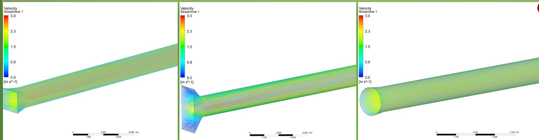
Comparative CFD study on different shapes of bell-mouths conducted for Rukumgadh Hydropower Plant
