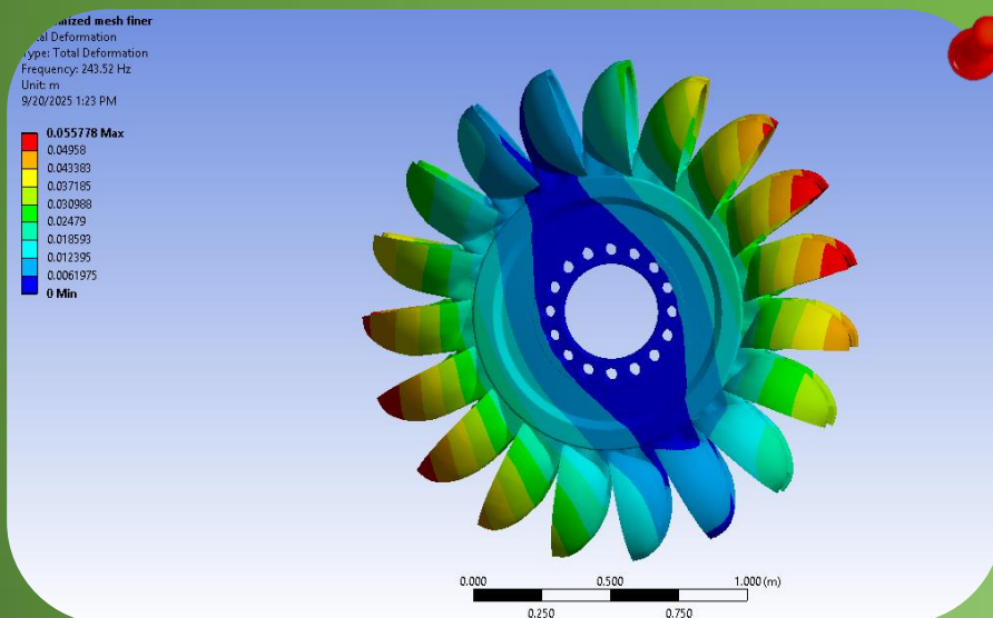
Modal analysis performed for the new 'Monsoon runner' design proposed by TTL for Mistri Khola Hydropower plant
