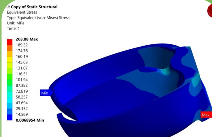
CFD and FEM analysis being conducted for the Pelton turbine buckets of Mistri Khola HPP as the part of agreement between KU and Mountain Energy Ltd.
