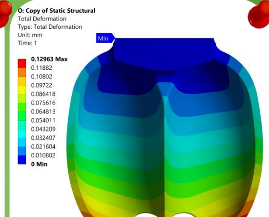
CFD and FEM analysis being conducted for the Pelton turbine buckets of Mistri Khola HPP as the part of agreement between KU and Mountain Energy Ltd.
